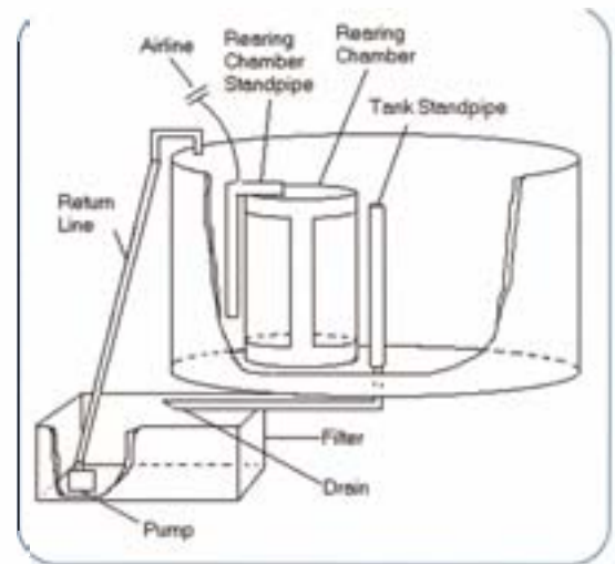
Fig. 4. Recirculating larval rearing system
