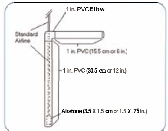
Fig. 6. Stand pipe used in the hatching and rearing chamber
