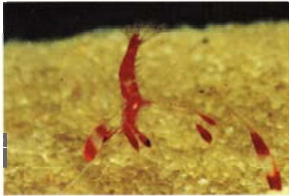
Fig. 7 Fire shrimp post-larvae (day 68) with expanded fifth parapodia
