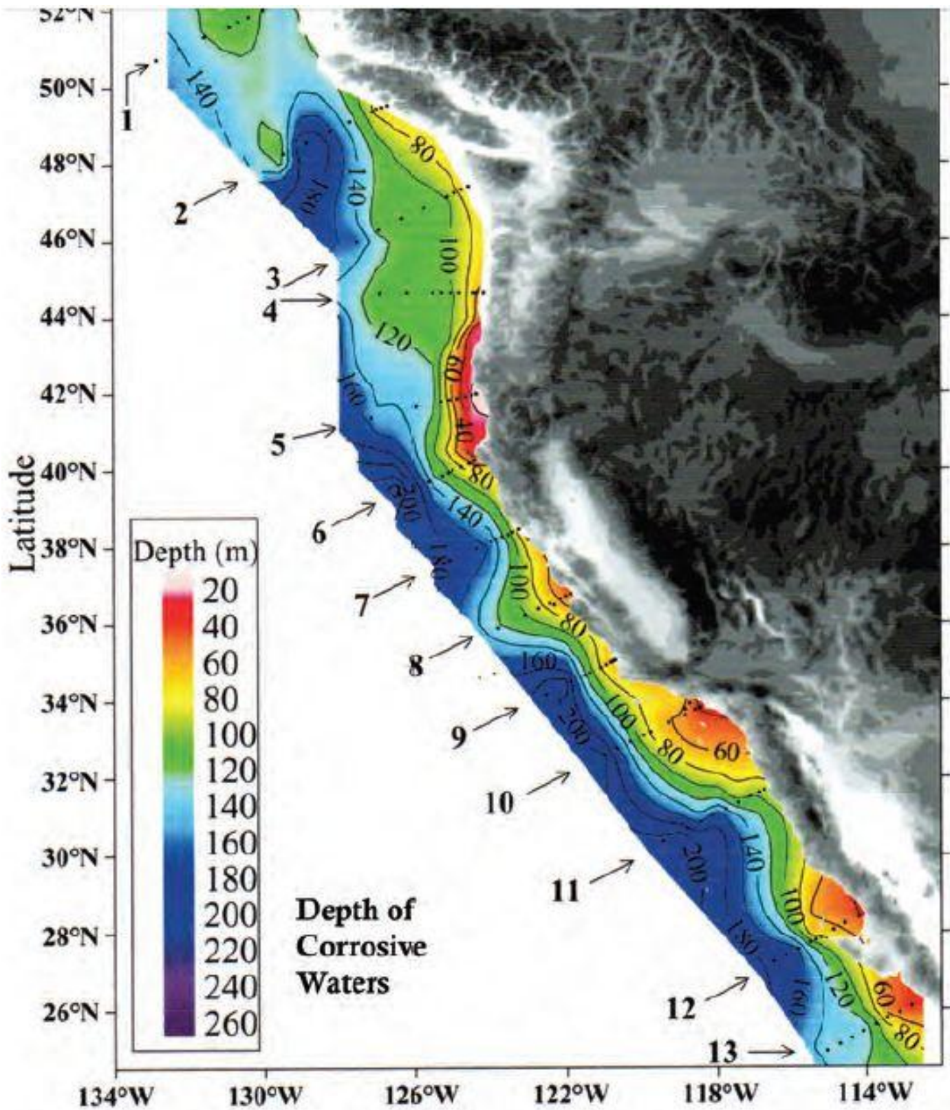
Depth of low-pH water, water understaturated with carbonate. From
