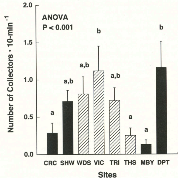
Figure 3. Human collecting activity at eight Orange County study sites (see fig. 1 for locations and abbreviations; after Murray 1998). Filled bars indicate longstanding, signed CMLRs; cross-hatched bars designate nonreserve sites (prior to 1994). Signs indicating CMLR status were not posted at nonreserve study sites given protection on January 1, 1994, until after all our data were collected. Plotted values represent the annual mean number of collectors (+1 SE) for each site calculated from the twelve monthly averages obtained between February 1995 and January 1996. Mean values designated by the same letter (a or b) belong to the same subset on the basis of the Student-Newman-Keuls (SNK) a posteriori multiple comparison test.
